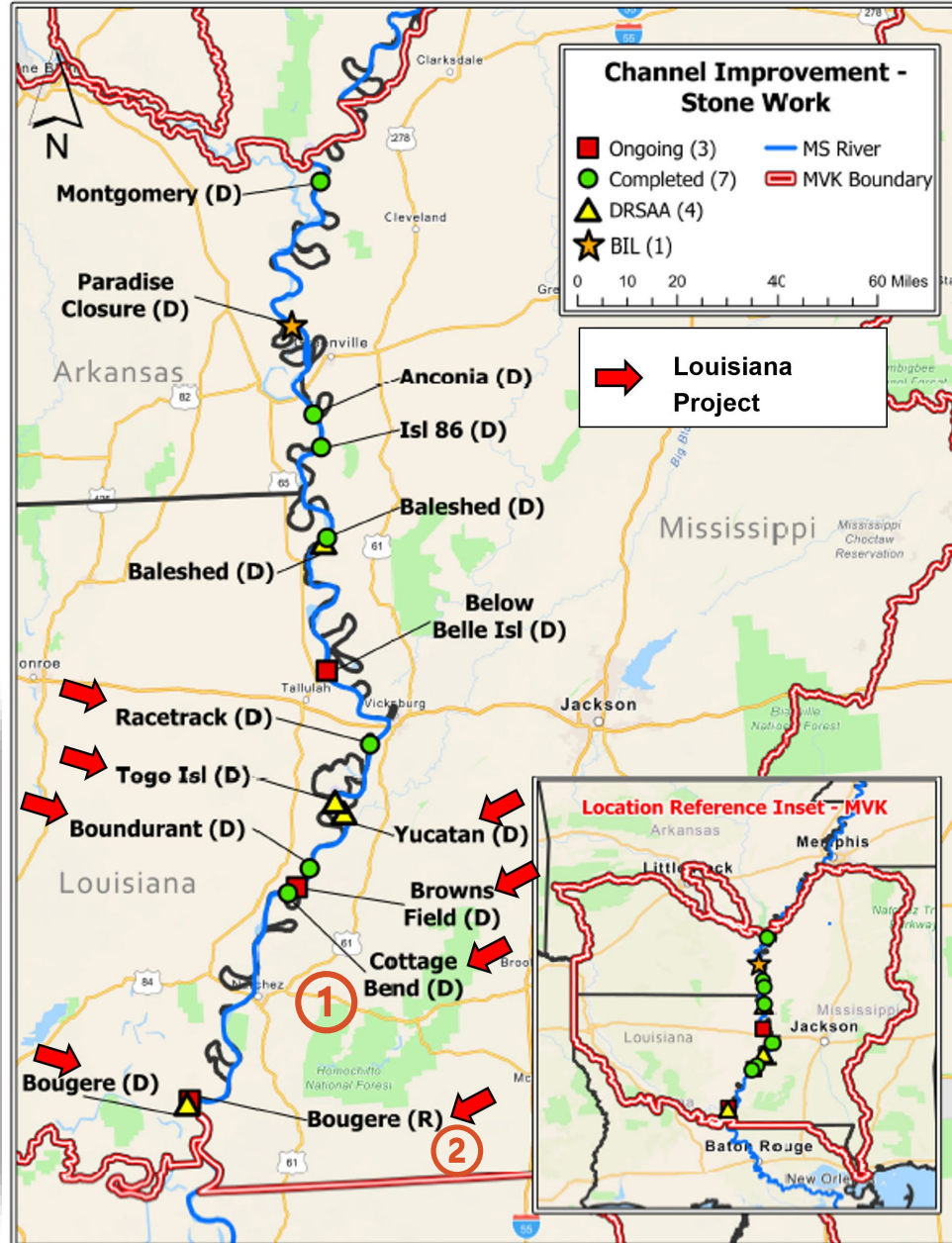
Dike maintenance, Cottage Bend Dike 3L, RM 388
